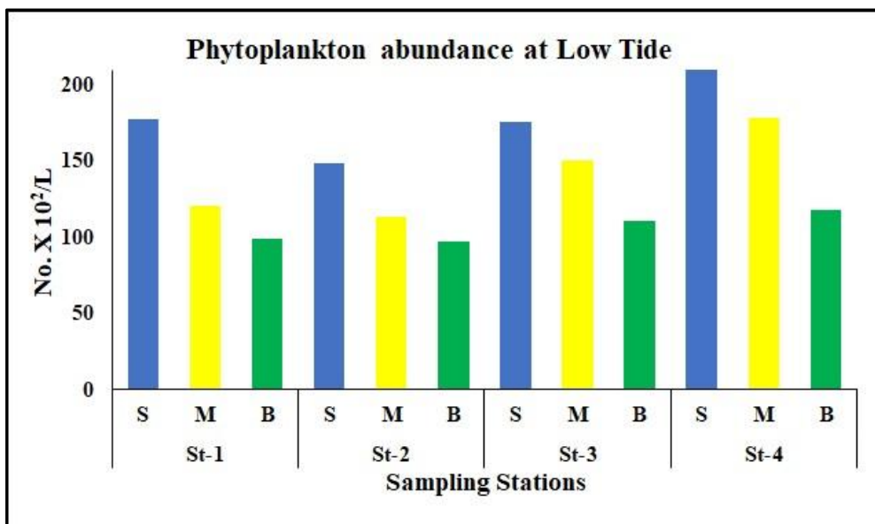
Figure 10: Low Tidal Level (LTL) phytoplankton abundance (no. x10 2 / L) at different sampling stations at Petronet LNG, Dahej during December 2024
