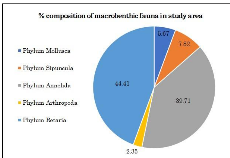
Figure 7: Percent composition of Subtidal benthic taxa from the marine waters of Petronet LNG, Dahej during December 2024
